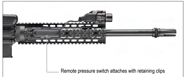
Ergonomic push-button switch Remote switch exits port at 90° providing improved cable routing to preserve rail space
